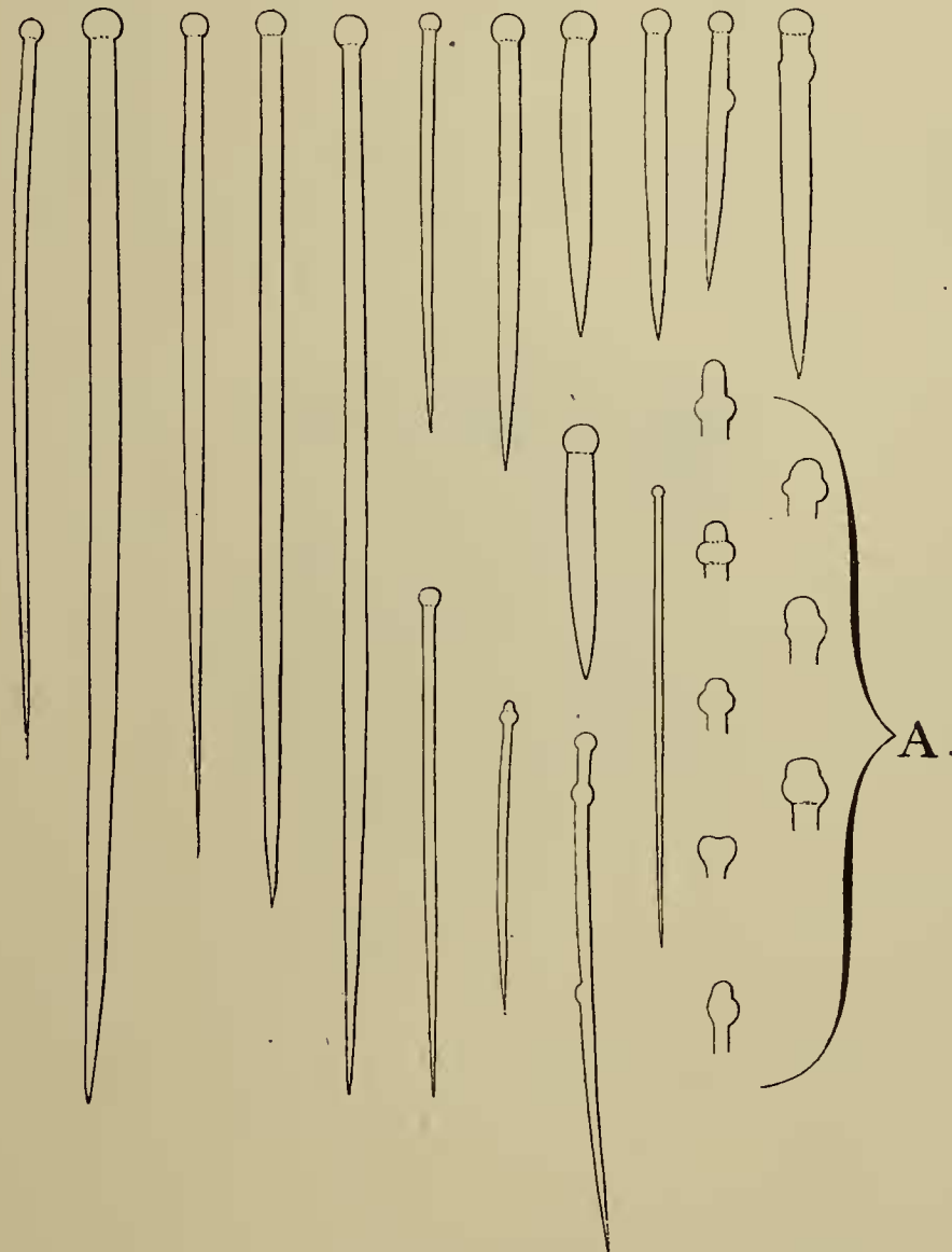
FIG. 5.— Suberites sericeus , Thiele. Spicules of a specimen in phase B, \times 255 . A.—Heads of spicules further enlarged.
